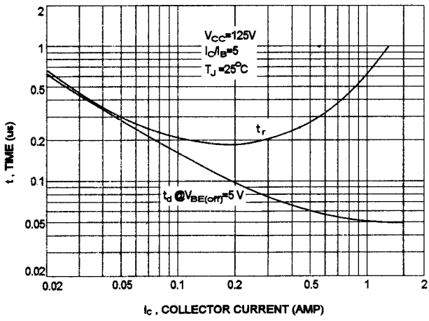
TURN-ON TIME
